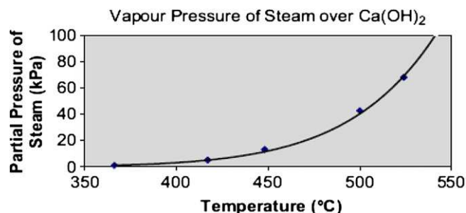
Fig. 4. Partial pressure of water vapour over Ca(OH) 2 .
